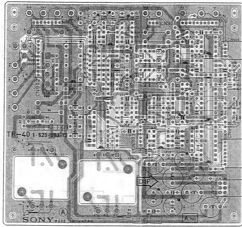
1-620-903-13 COMPONENT SIDE
